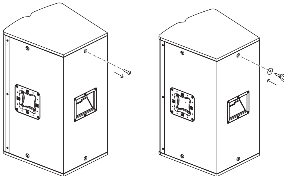
Figure 4.2: Removing the M10 screws and installing the fender washers and eyebolts
