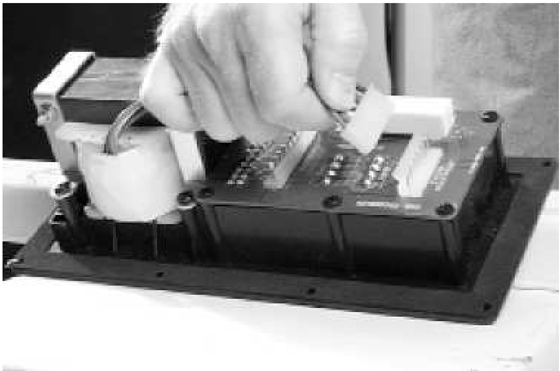
Figure 6.5: EVA input panel with EVA-AM installed showing connector plug-in
