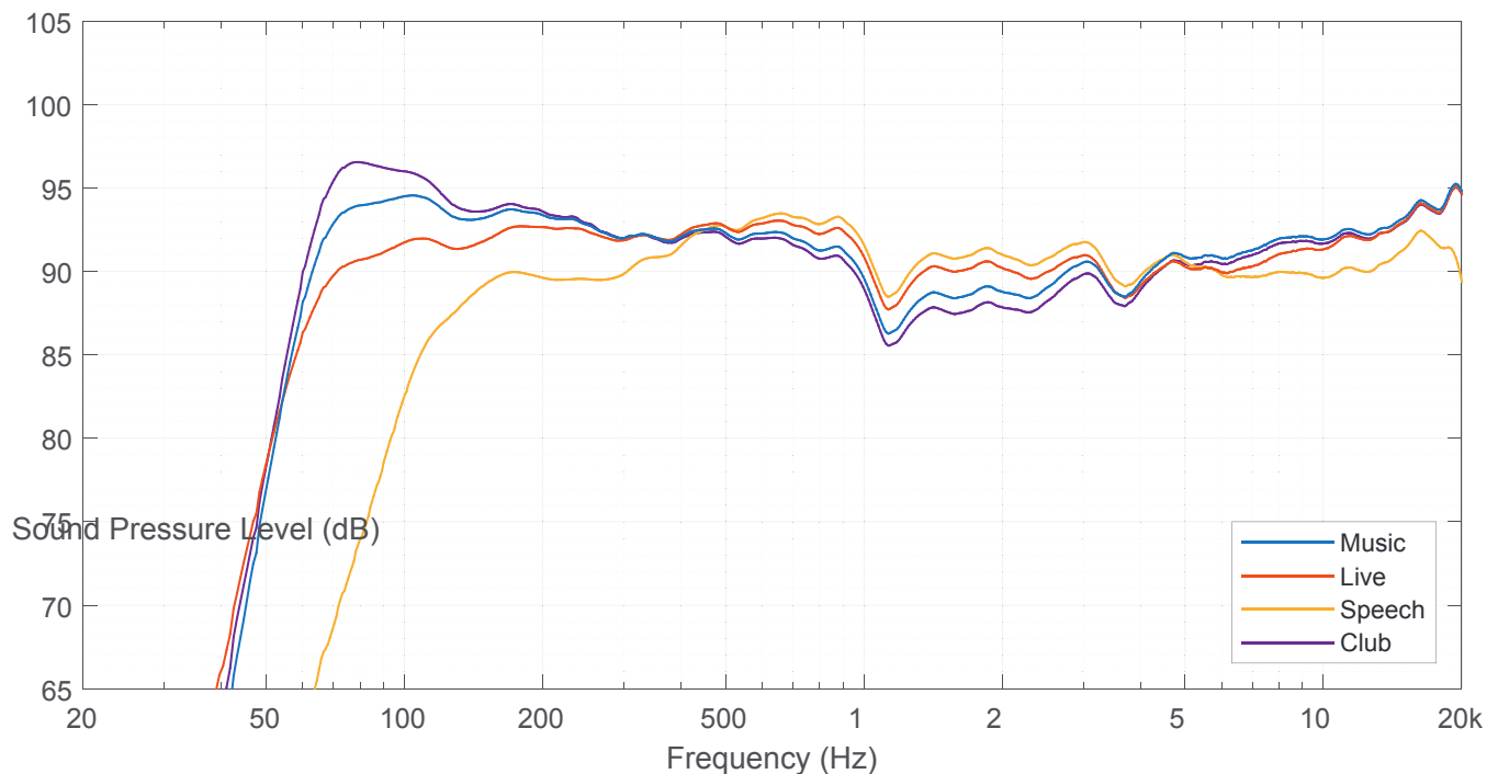
Fig. 2: Frequency response
