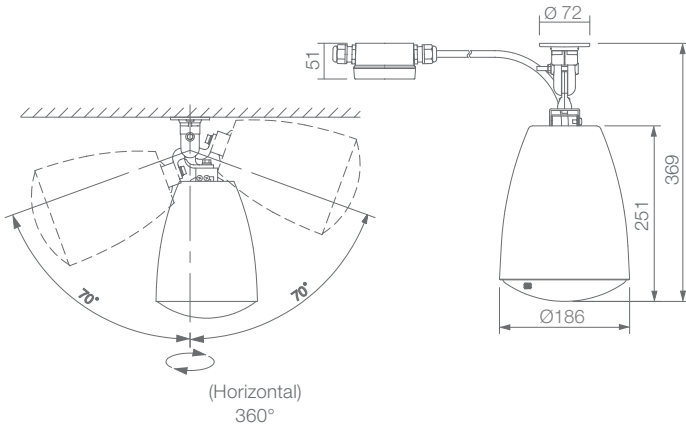
PE-154EN/ PE-154EN-BK
