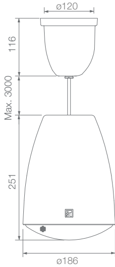
PE-154EN-BS
