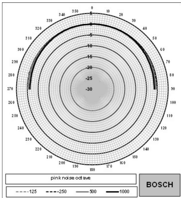
Fig. 2: Polar diagram LCM-30CW-R low frequency part (frequency in Hz)
