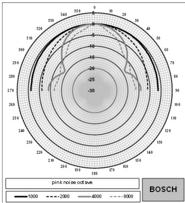
Fig. 1: Polar diagram LCM-30CW-R high frequency part (frequency in Hz)
