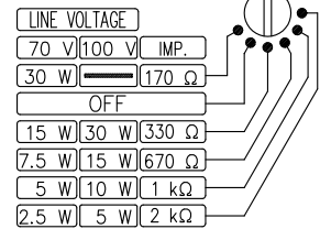
Impedance selection
