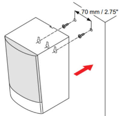
Fig. 2: LB1-UW06-x1 wall mounting
