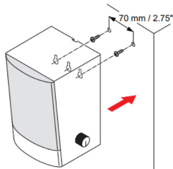
Fig. 3: LB1-UW06V-x1 wall mounting
