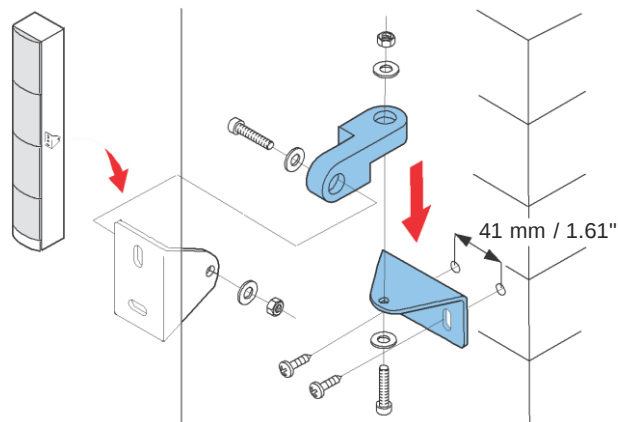
Mounting of the wall- and turn brackets.
