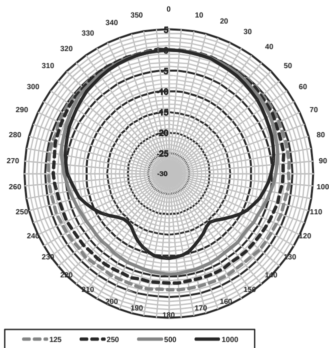
LA1-UW24-x1 polar diagram horizontal (low frequency)
